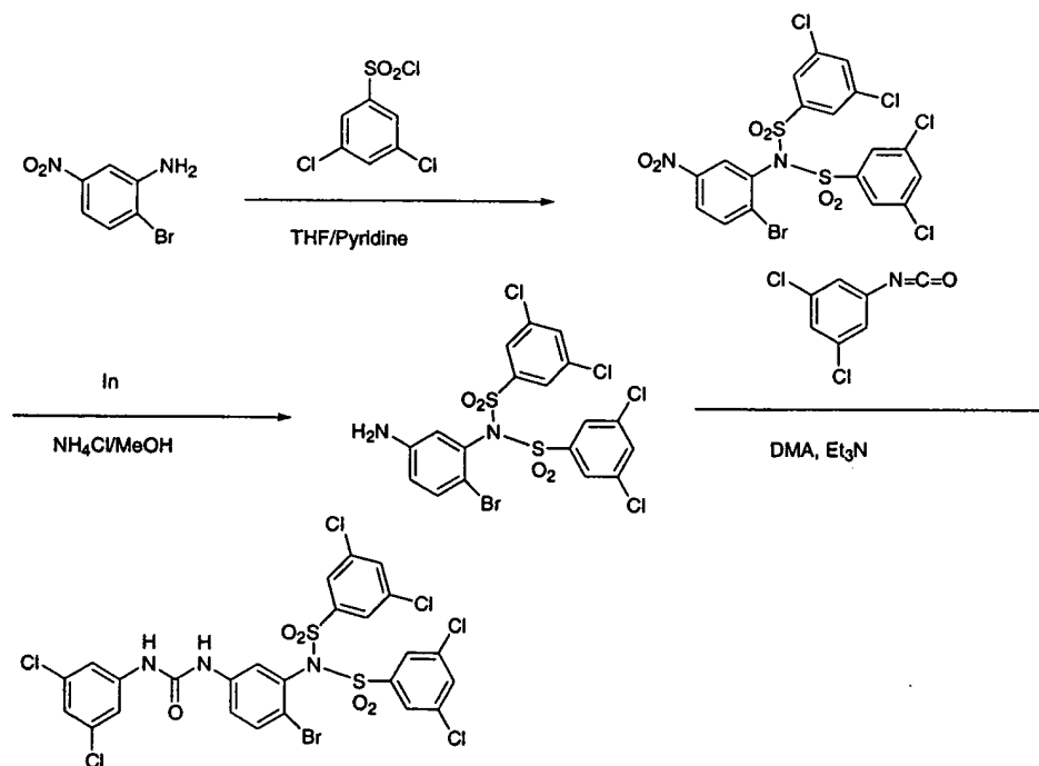
Scheme IV-C
